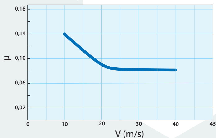
Coefficient of friction ( \mu ) at a current density of 14 A/cm 2
