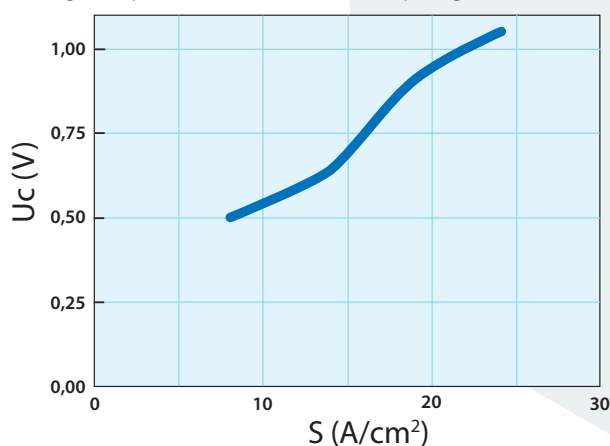
Voltage drop ( U_c ) between brush & slip ring at 18 m/s
